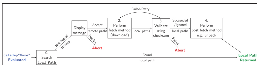
Figure 2: The process that is executed when a data dependency is accessed by name.
