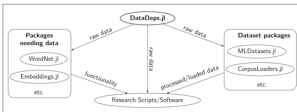
Figure 1: The current package ecosystem depending on DataDeps.jl.
