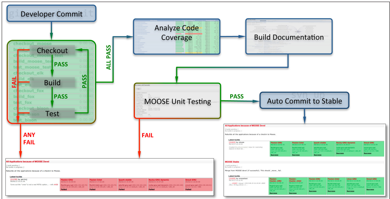
Figure 1: Flowchart depicting the MOOSE project's automatic build and testing system. After a developer commits a change, MOOSE and all the applications are built and tested. If any test fails, the system exits and reports failure. Otherwise, once all tests have succeeded, “stable” MOOSE is automatically updated, making it available to users.
