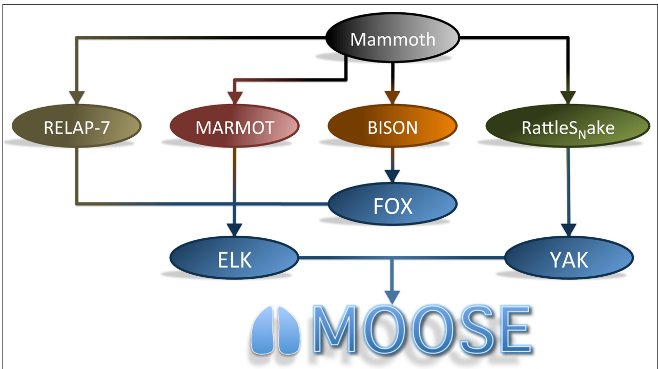
Figure 2: Flowchart of automated dependency build system for MOOSE and applications.
