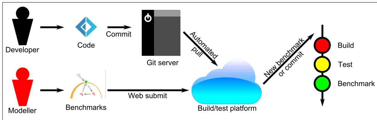
Figure 2: Proposed reproducibility service workflow.
