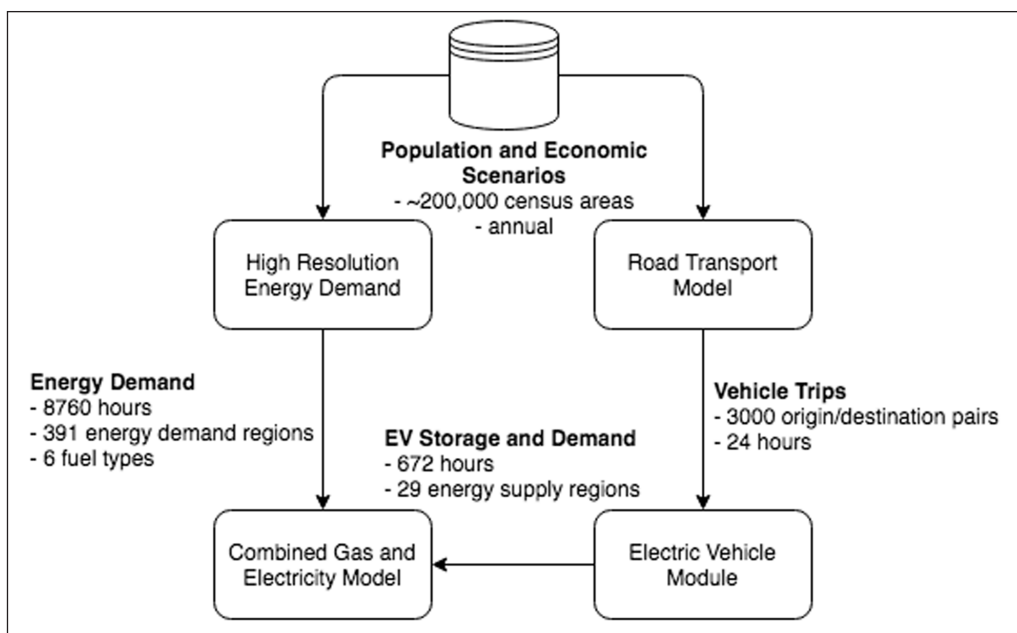
Figure 1: A sketch of the diverse data dimensions produced and required by energy and transport models – a subset of the infrastructure simulation models included in NISMOD 2.
